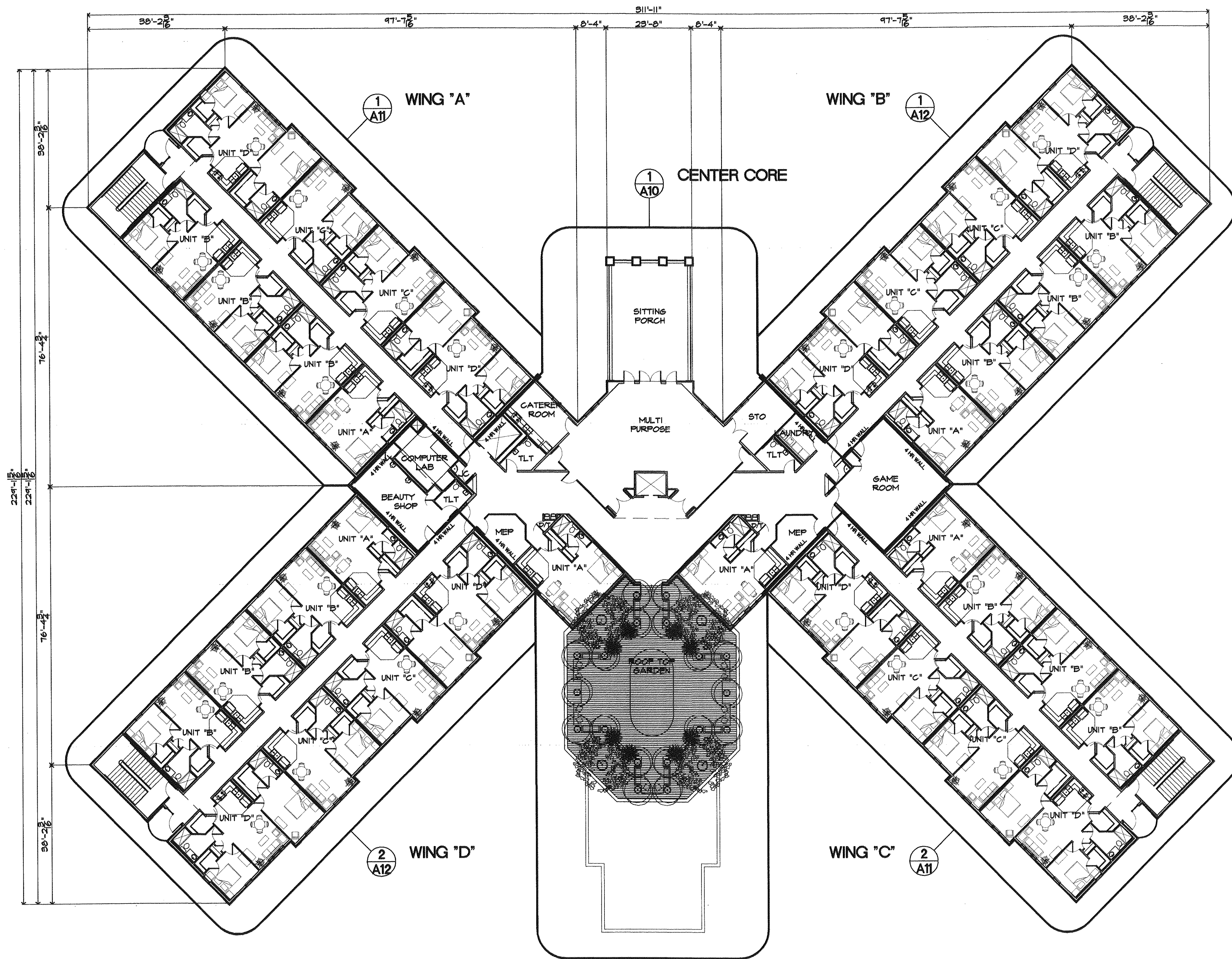
AREA = 91,916 sq. ft. 1 A3 THIRD FLOOR PLAN SCALE: 1/16" = 1'-0" NORTH
