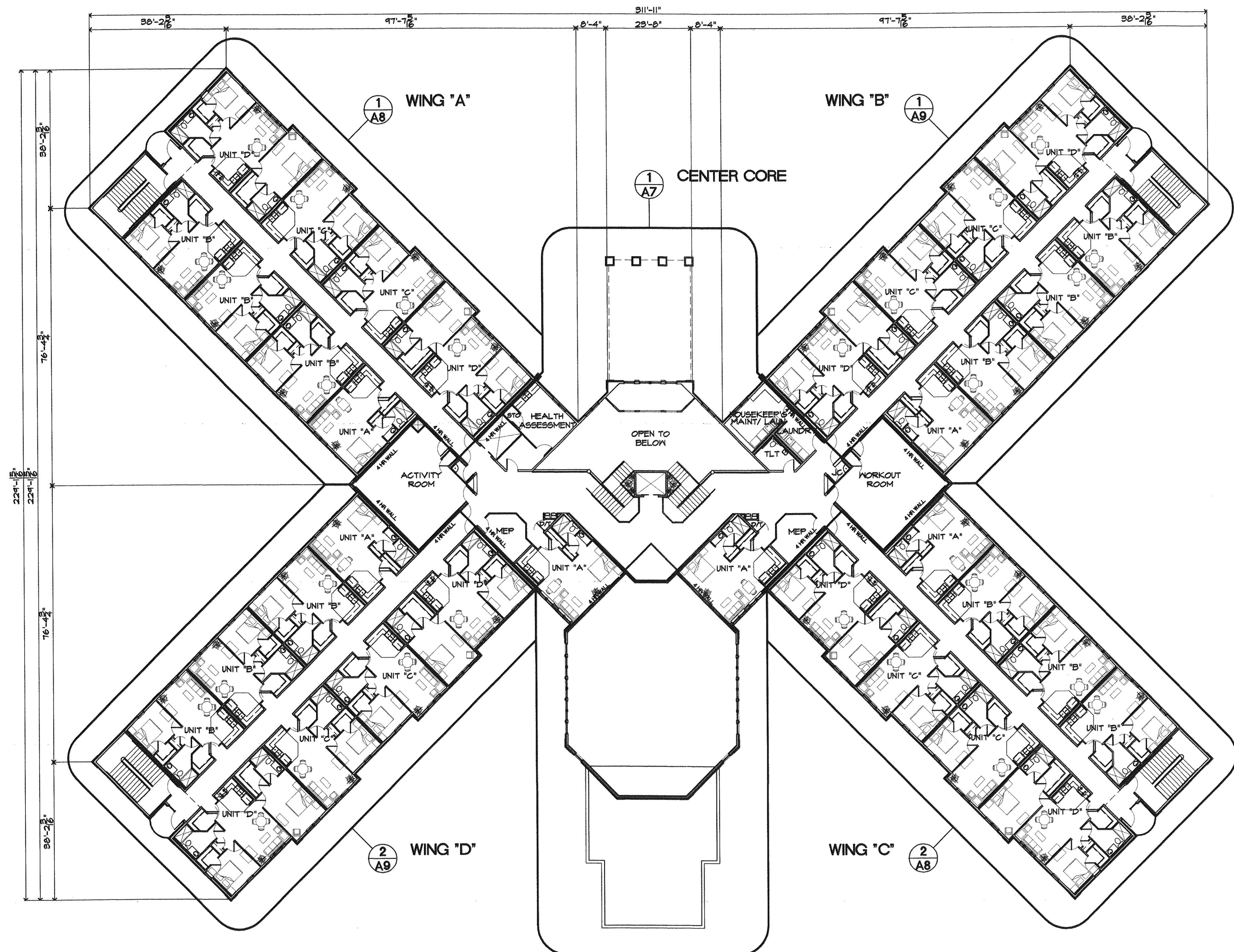
AREA = 29,940 sq. ft. 1 A2 SECOND FLOOR PLAN SCALE: 1/16" = 1'-0" NORTH
